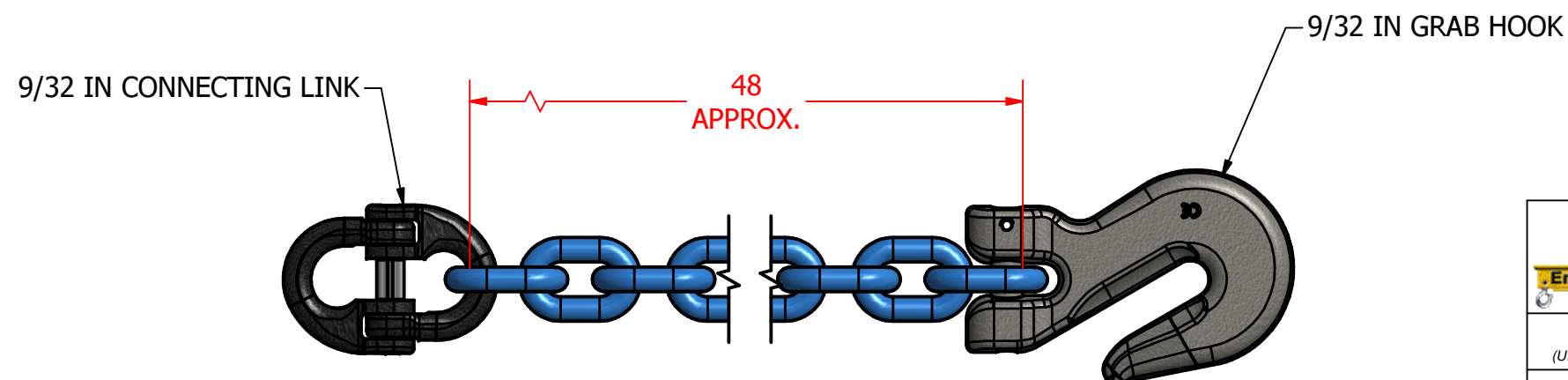
SAFETY CHAIN ASSEMBLY 2 INCLUDED
